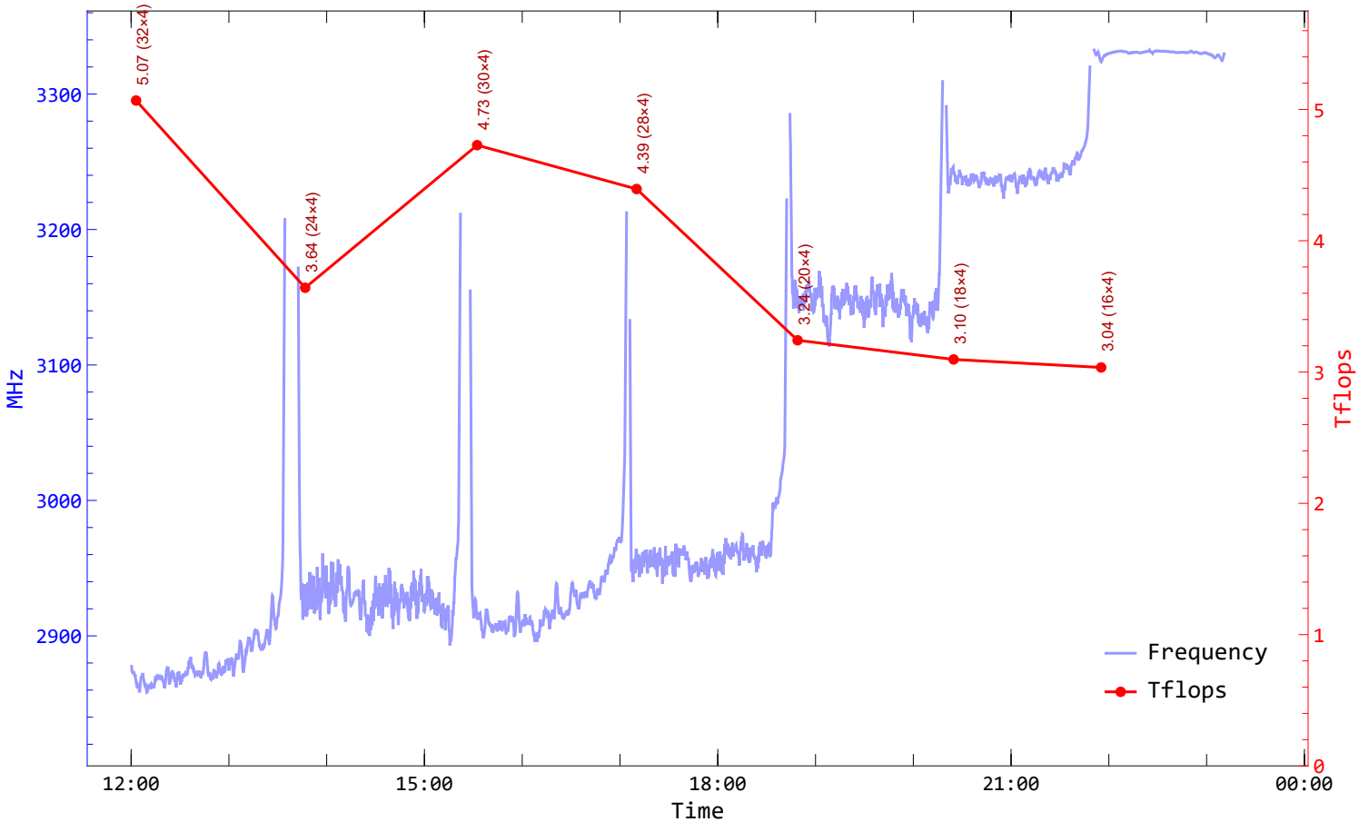
HPL, NB = 224, N ~ 1000 TB - Frequency and Tflops over time (node = c03n[03-04])
