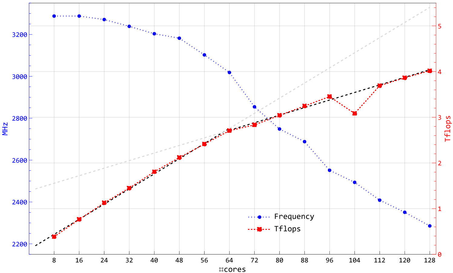
HPL, NB = 224, N ~ 1000TB – Frequency and Tflops vs #cores (avgs for 6x R6525 7H12)
