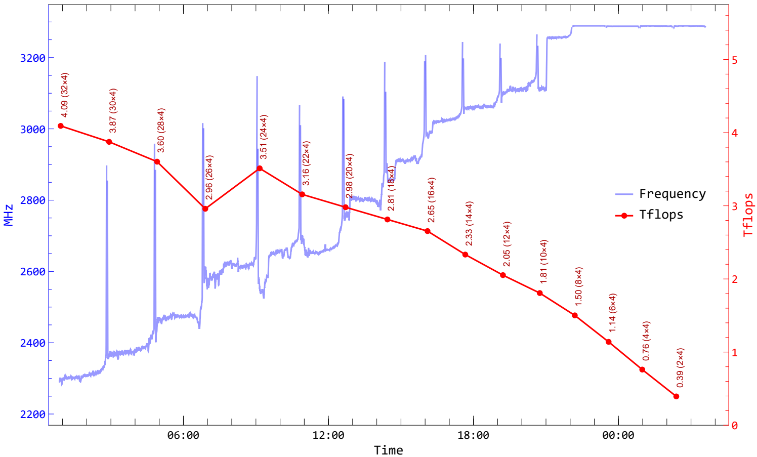
HPL, NB=224, N~1000TB – Frequency and Tflops over time (node=c04n06)
