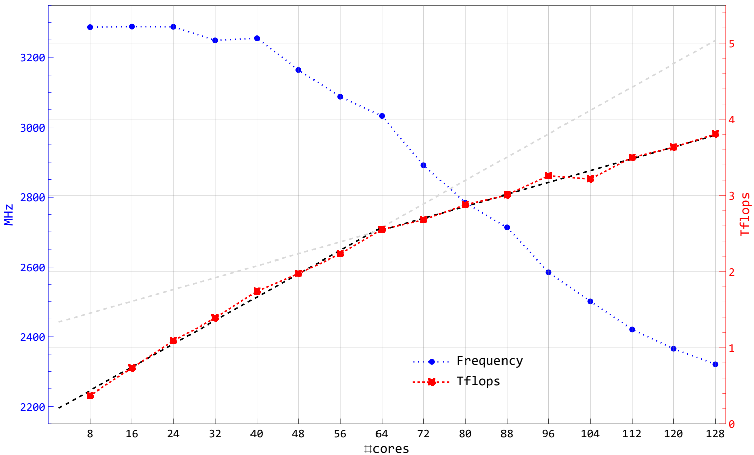
HPL, NB=224, N~250MB – Frequency and Tflops vs #cores (avgs for 6x R6525 7H12)
