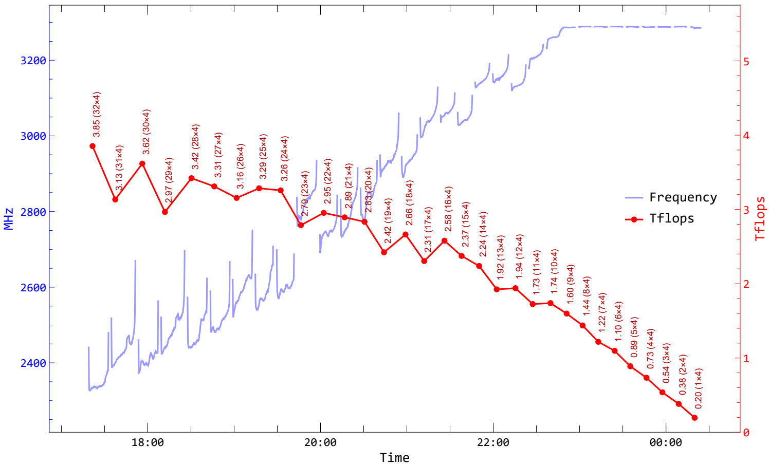
HPL, NB = 224, N ~ 250MB – Frequency and Tflops over time (node = c04n06)
