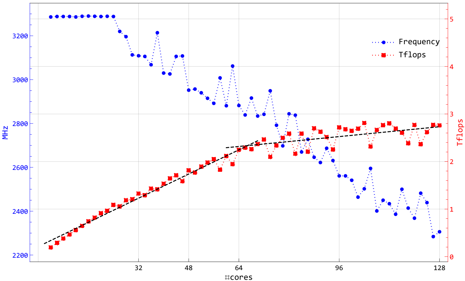
HPL, NB = 128, N = 82816, Frequency and Tflops vs #cores; node c04n06 (R6525 7H12)
