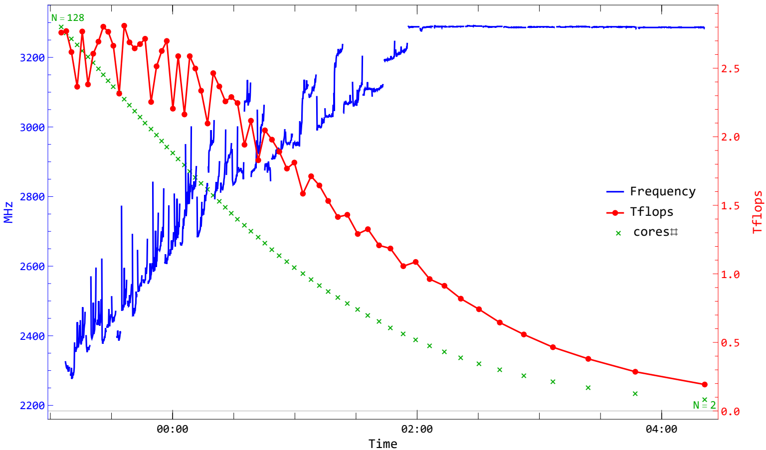
HPL, NB=128, N=82816, Frequency, Tflops and #cores over time
