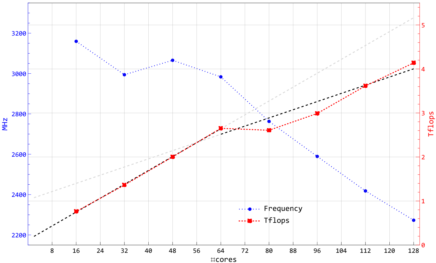
7H12, NB = 224, omp=8, N = 351680 (scaled) – Frequency and Tflops vs #cores (c04n[01-06] avg)
