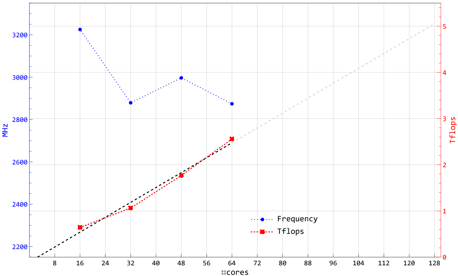
7502, NB = 224, omp=8, N = 248640 (scaled) – Frequency and Tflops vs #cores (c03n03)
