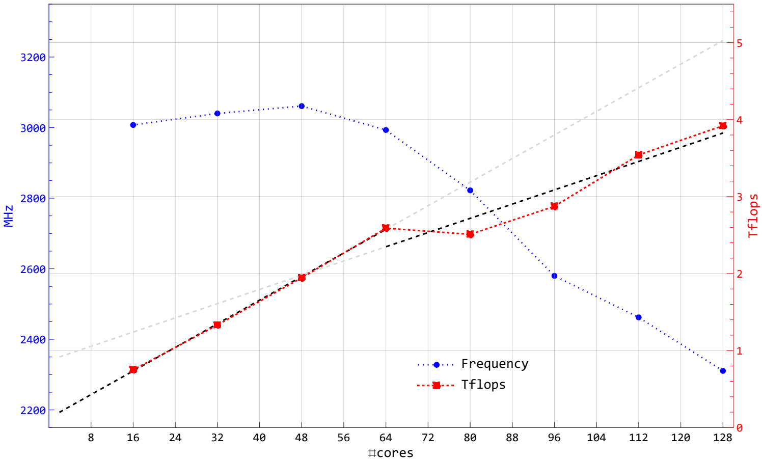
7H12, NB = 224, omp=8, N=173824 (scaled) – Frequency and Tflops vs #cores (node206)
