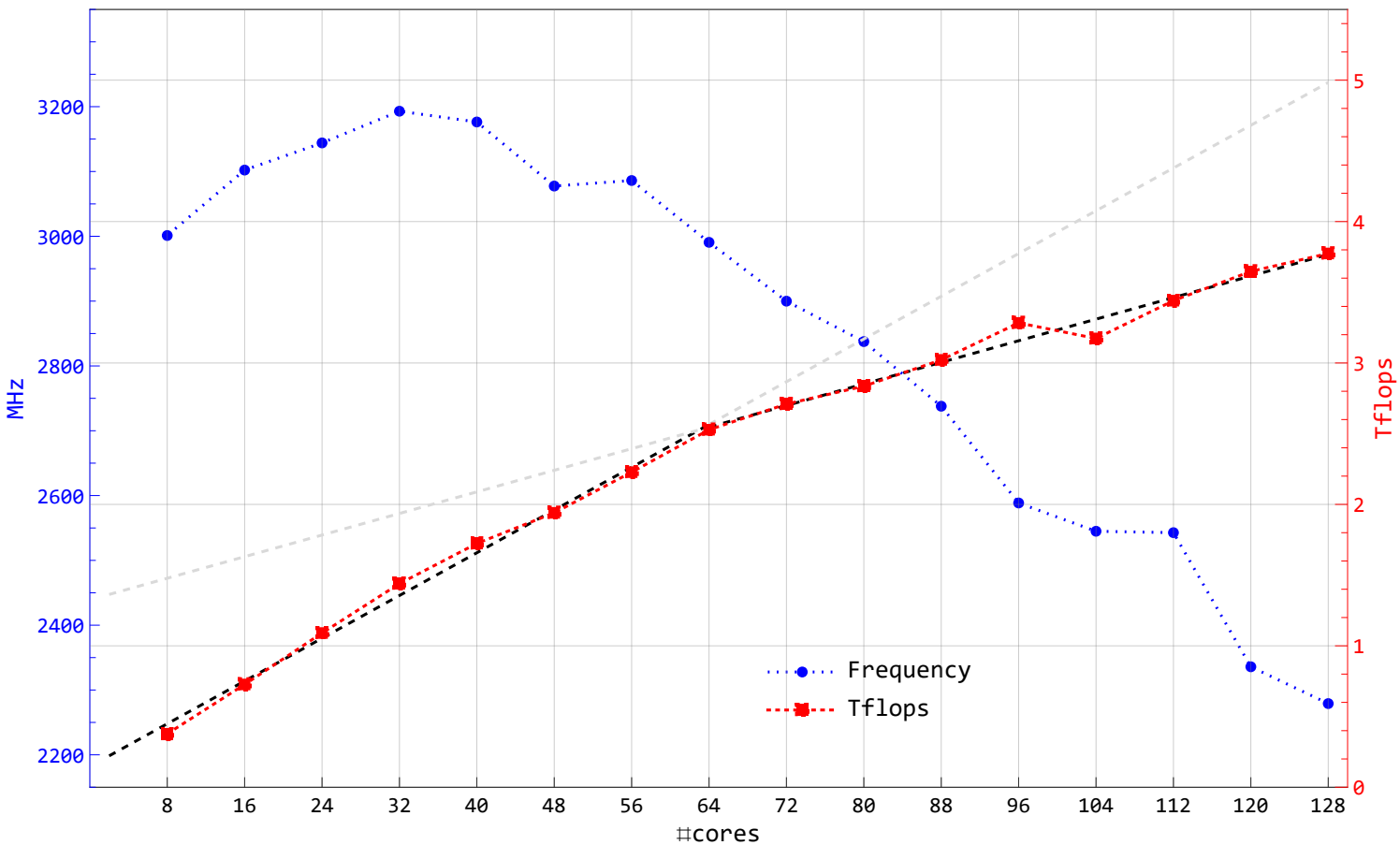
7H12, NB = 224, N = 173824 (scaled) – Frequency and Tflops vs #cores (node206)
