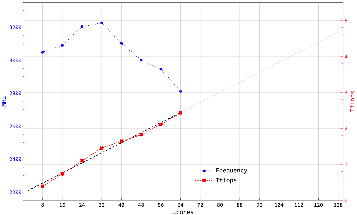
7502, NB = 224, N = 173824 (scaled) – Frequency and Tflops vs #cores (node202)
