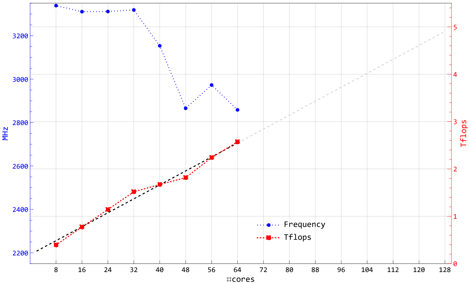
HPL, NB = 224, N ~ 500 TB – Frequency and Tflops vs #cores (avgs for 2x R6525 7502)
