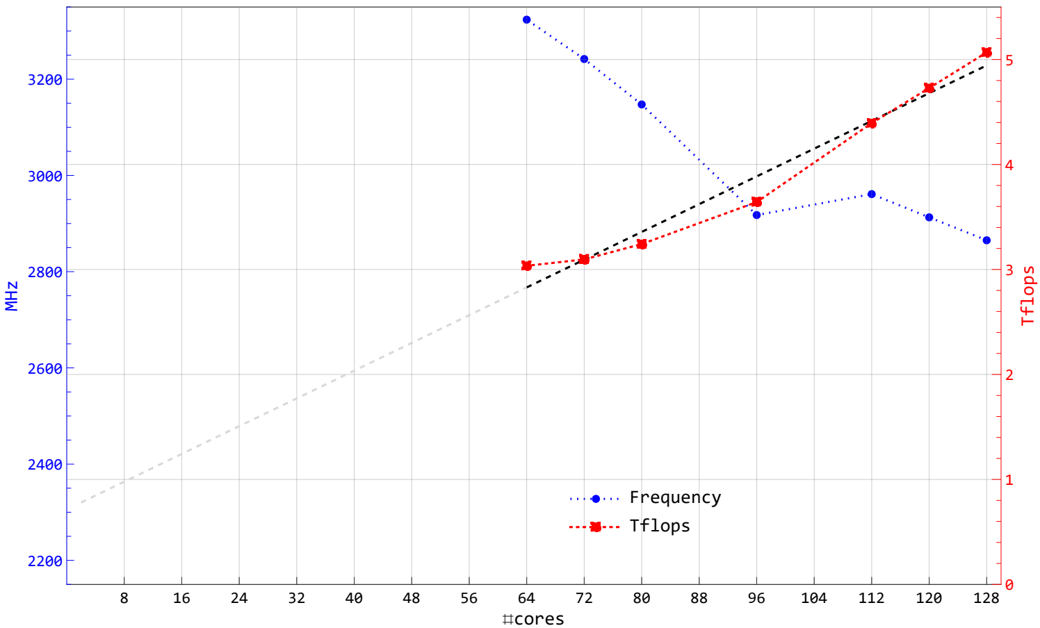
HPL, NB=224, N~1000 TB – Frequency and Tflops vs #cores (2x R6525 7502 over Infiniband)
