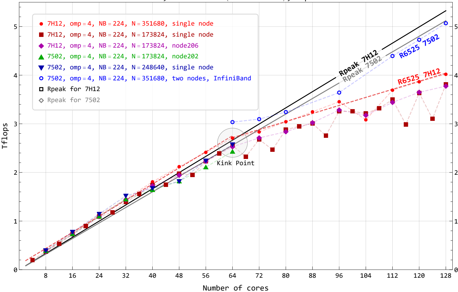
HPL, Performance (7H12 vs 7502), omp = 4
