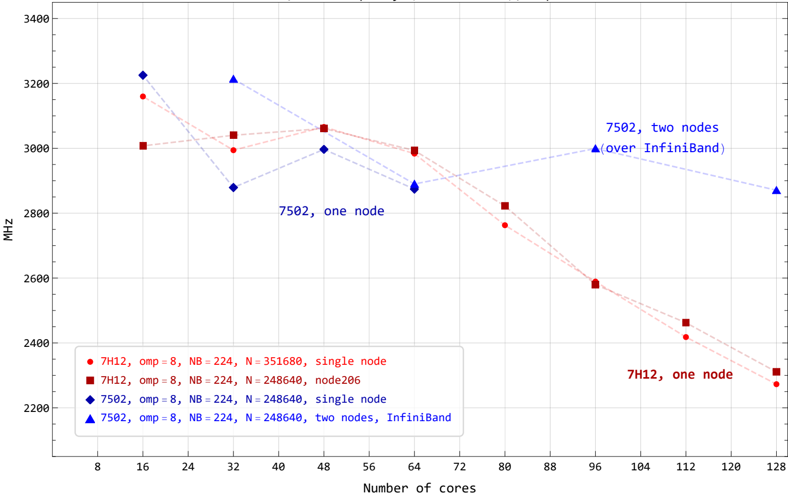
HPL, CPU frequency (7H12 vs 7502), omp = 8
