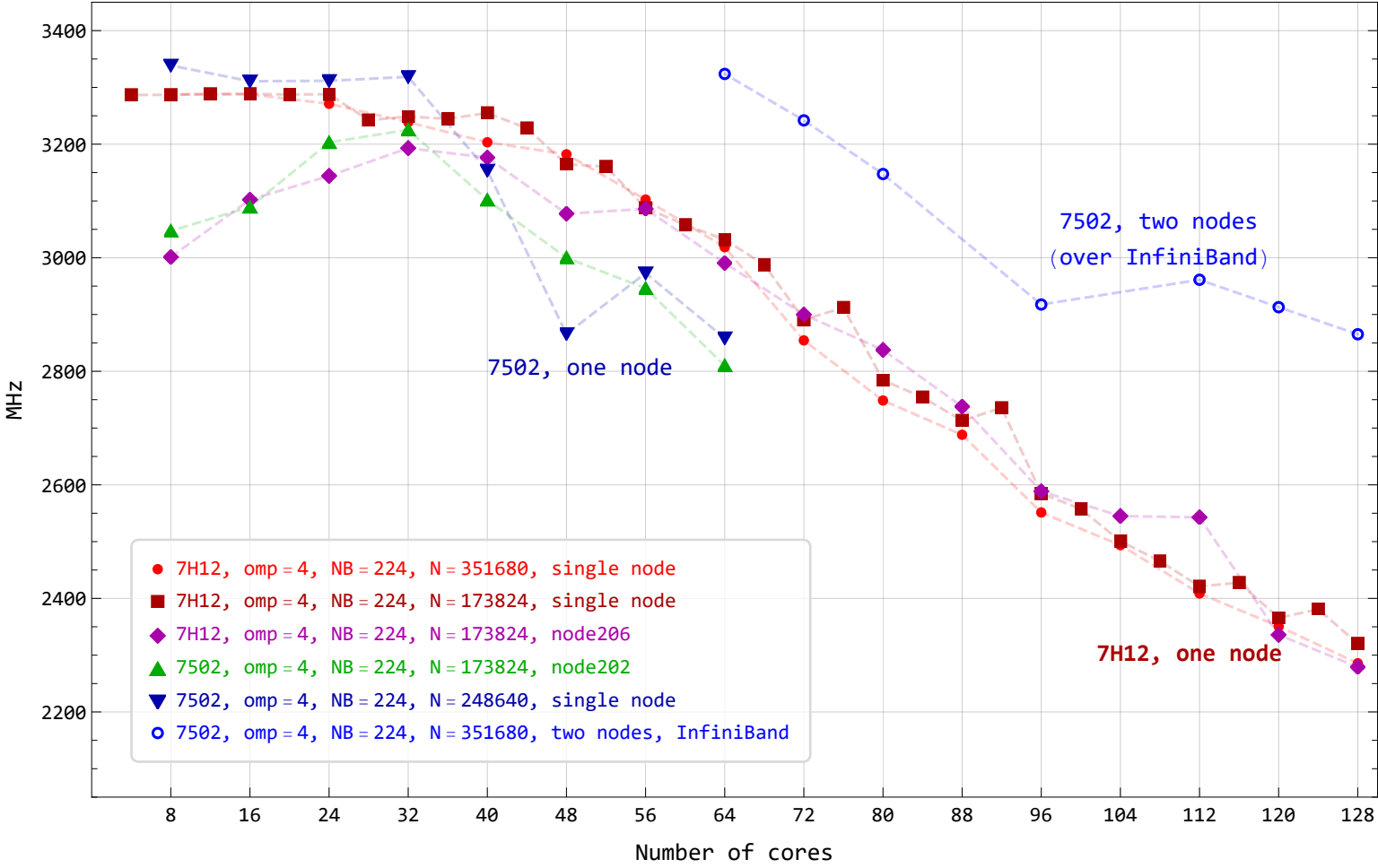
HPL, CPU frequency (7H12 vs 7502), omp = 4
