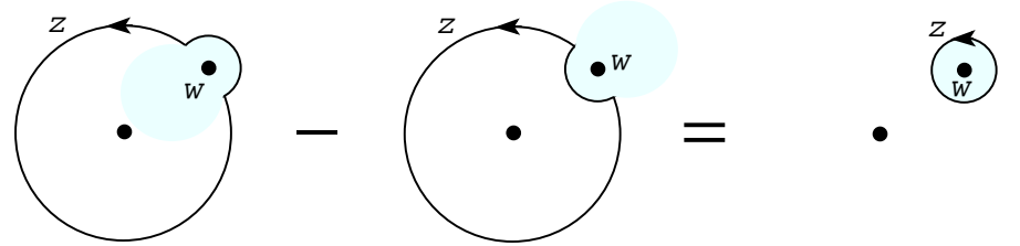
Fig. 2. Evaluation of “equal-time” commutator on the conformal plane.
